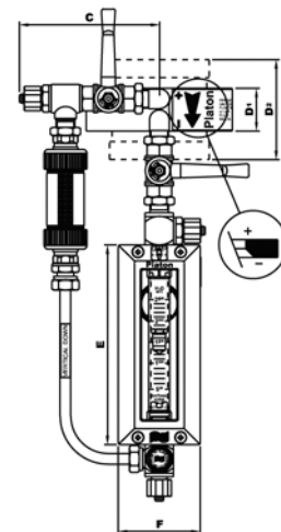
VERTICAL FLOW DOWNWARDS
